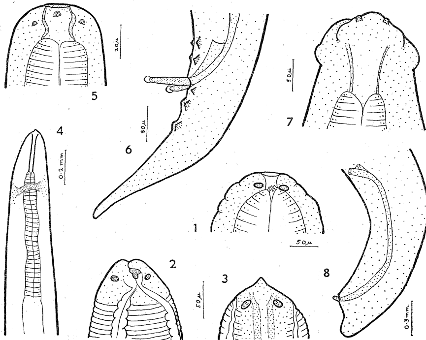
Figs. 1-8.—1. Denticulospirura dentata ; 1. head. 2-4. Acuaria corvicola ; 2. head, ventral view; 3. head, lateral view; 4. anterior end. 5-6. Oxyspirura streperae ; 5. head of female; 6. male tail. 7-8. Spironoura elseyae ; 7. head; 8. male tail. Figs. 2 and 3 to same scale.
