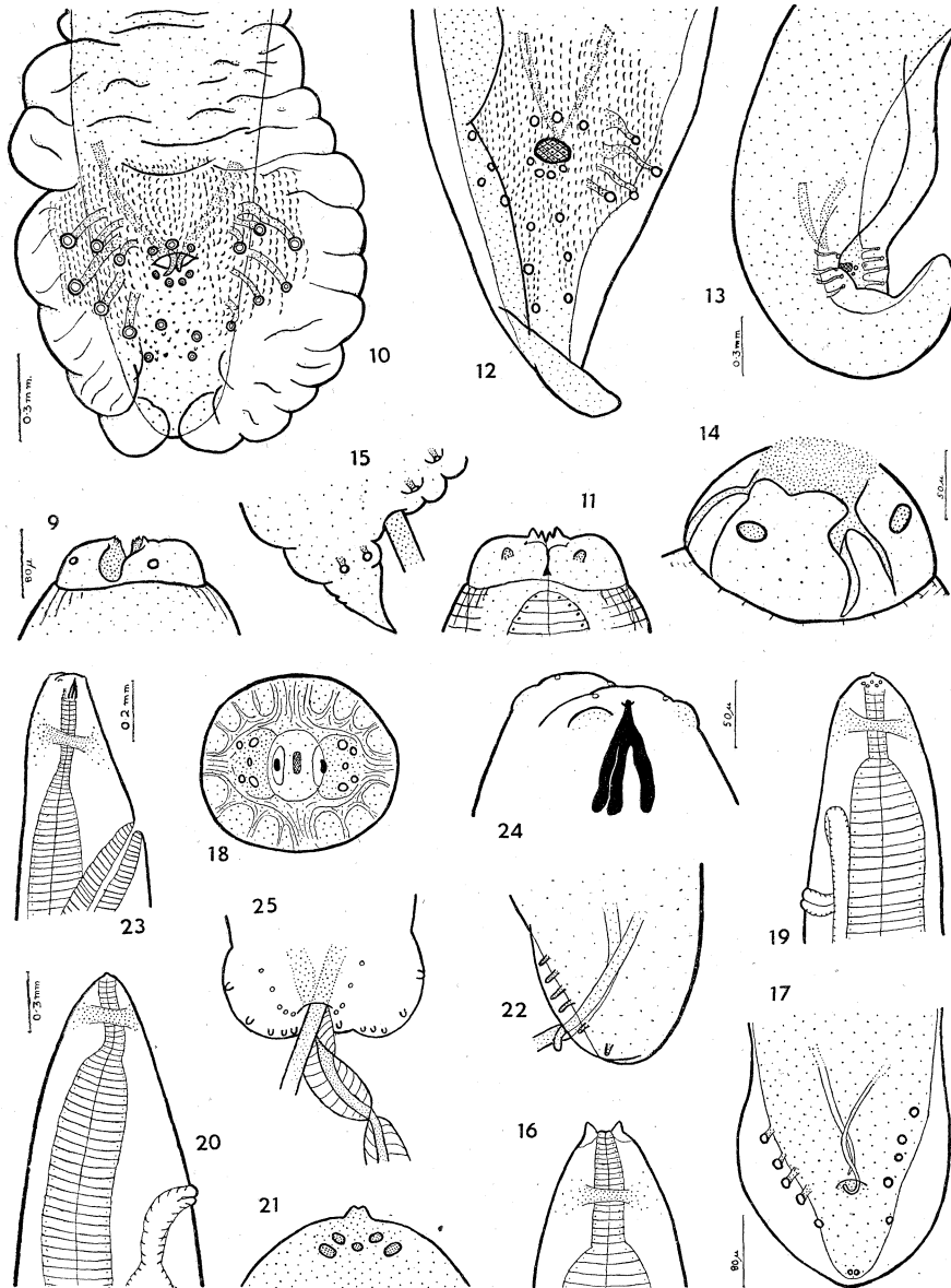
Figs. 9-25.—9-10. Physaloptera banfieldi ; 9. head of female; 10. bursa of male. 11-13. Physaloptera trougtoni ; 11. head; 12. posterior end of male, ventral view, one of alae folded over tail; 13. complete bursa, lateral view. 14-15. Contracaecum nycticoracis ; 14. head; 15. male tail. Figs. 9, 11 and 15 to same scale; Figs. 10 and 12. 16-17. Hamatospiculum mcneilli ; 16. anterior end of male; 17. male tail. 18-19. Hamatospiculum halcyonis ; 18. head of female, anterior view; 19. anterior end of female. 20-22. Hamatospiculum chibiae ; 20. anterior end of female; 21. head of male, lateral view; 22. male tail; 23-25. Diplotriaena tricuspis ; 23. anterior end of female; 24. head of female; 25. posterior end of male. Figs. 16, 19 and 23 to same scale; Figs. 17, 18, 22 and 25; Figs. 21 and 24.
